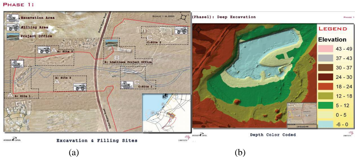
Figure 7: (a) Details of the Excavation and filling sites along the canal route within Phase I of the development area. (b) 3D color coded image of the excavation site 1 shown in (a).
