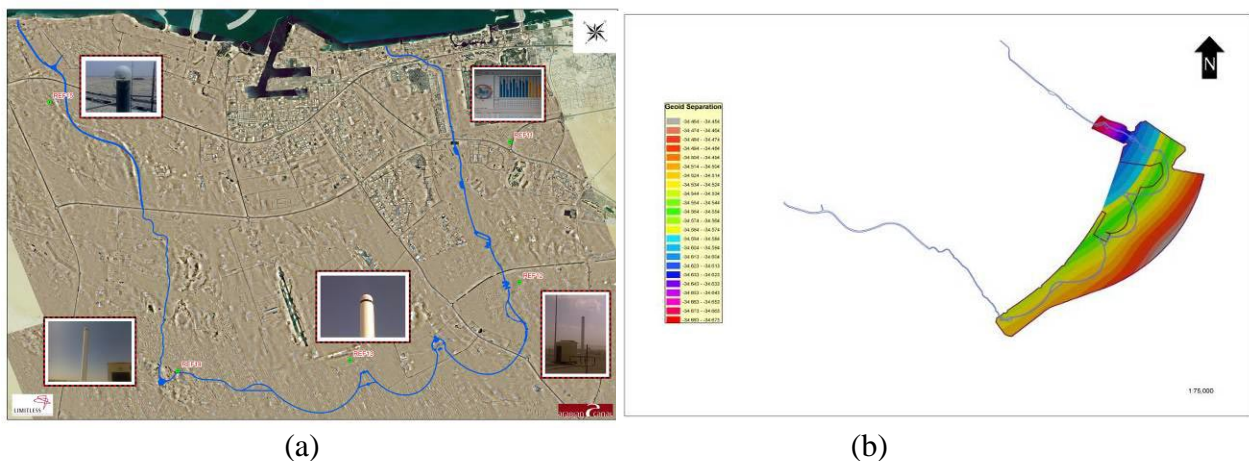
Figure 3: Vertical Datum modeling and Distribution of five GPS/GNSS reference stations around the Canal and development area. (a) Location of the GPS/GNSS reference stations (b) Geoids' Model to model of the development area.
