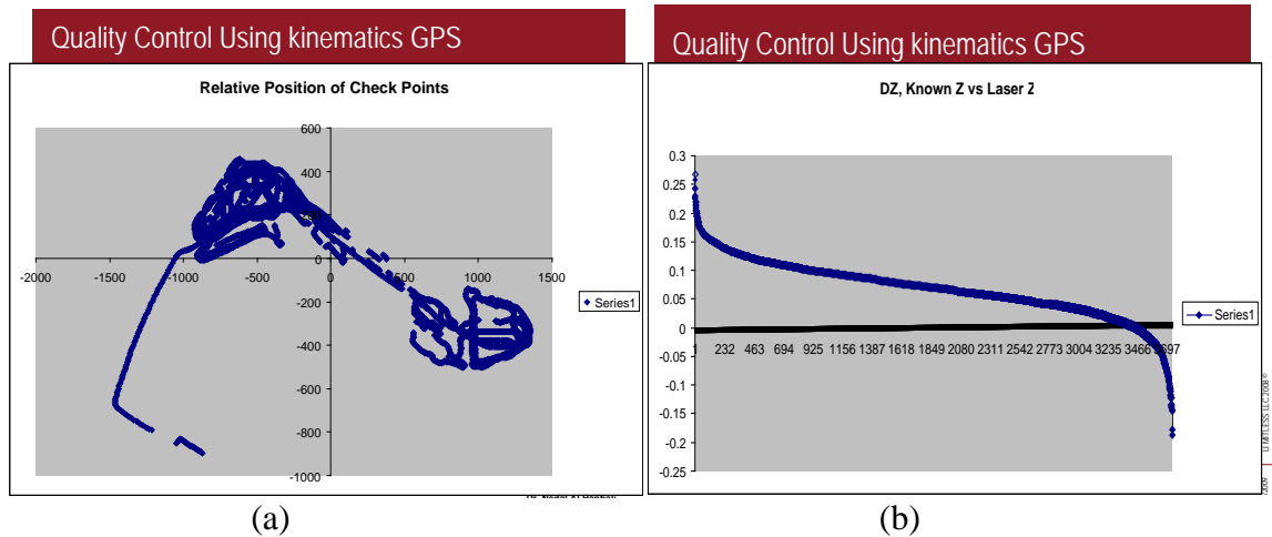
Figure 8: (a) the navigation route of the car with GPS antenna (b) vertical error variances of the generated DTM compared to GPS points.
